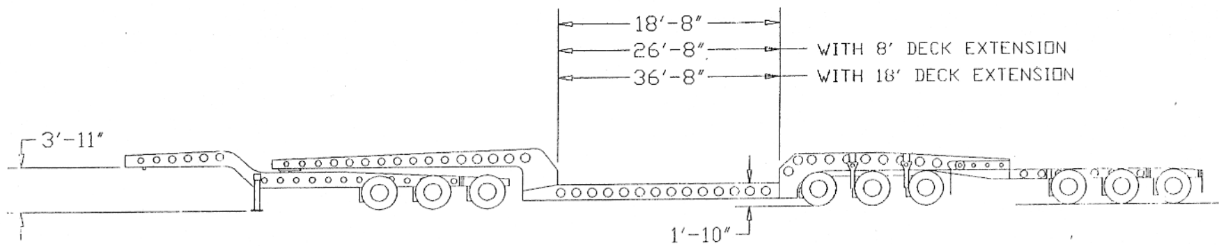
LOWBOY 9 AXLE - 160,000 L.B. CAPACITY
